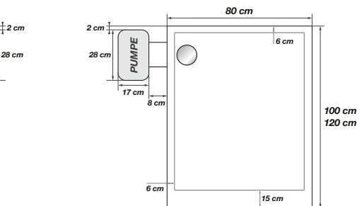
Pumpe links
